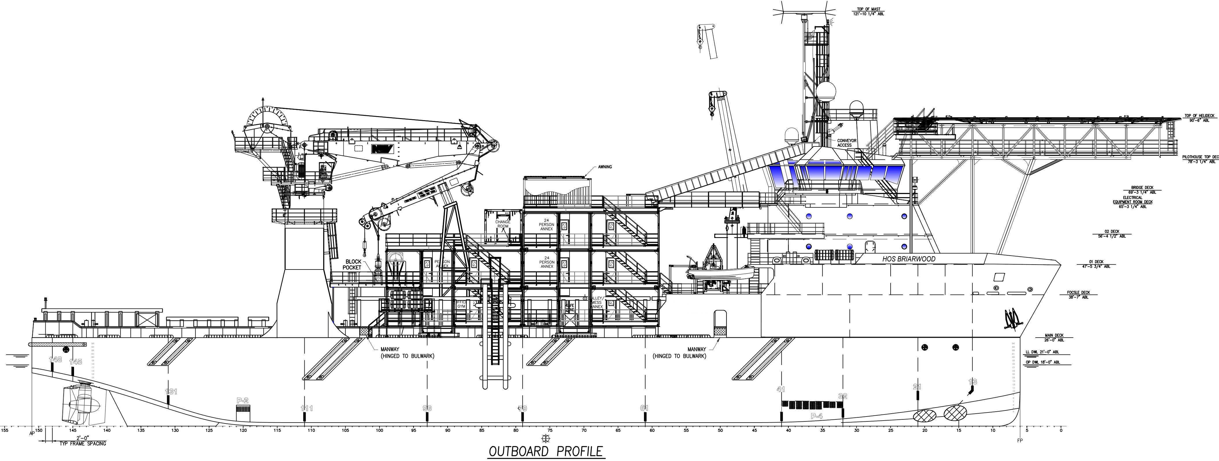
OUTBOARD PROFILE
