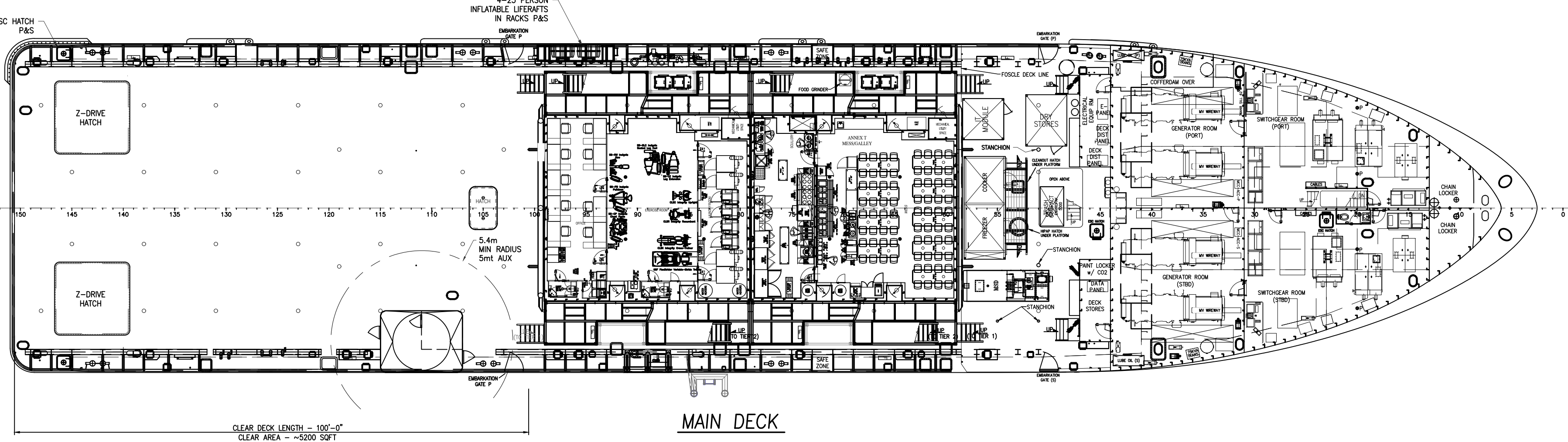
MAIN DECK
