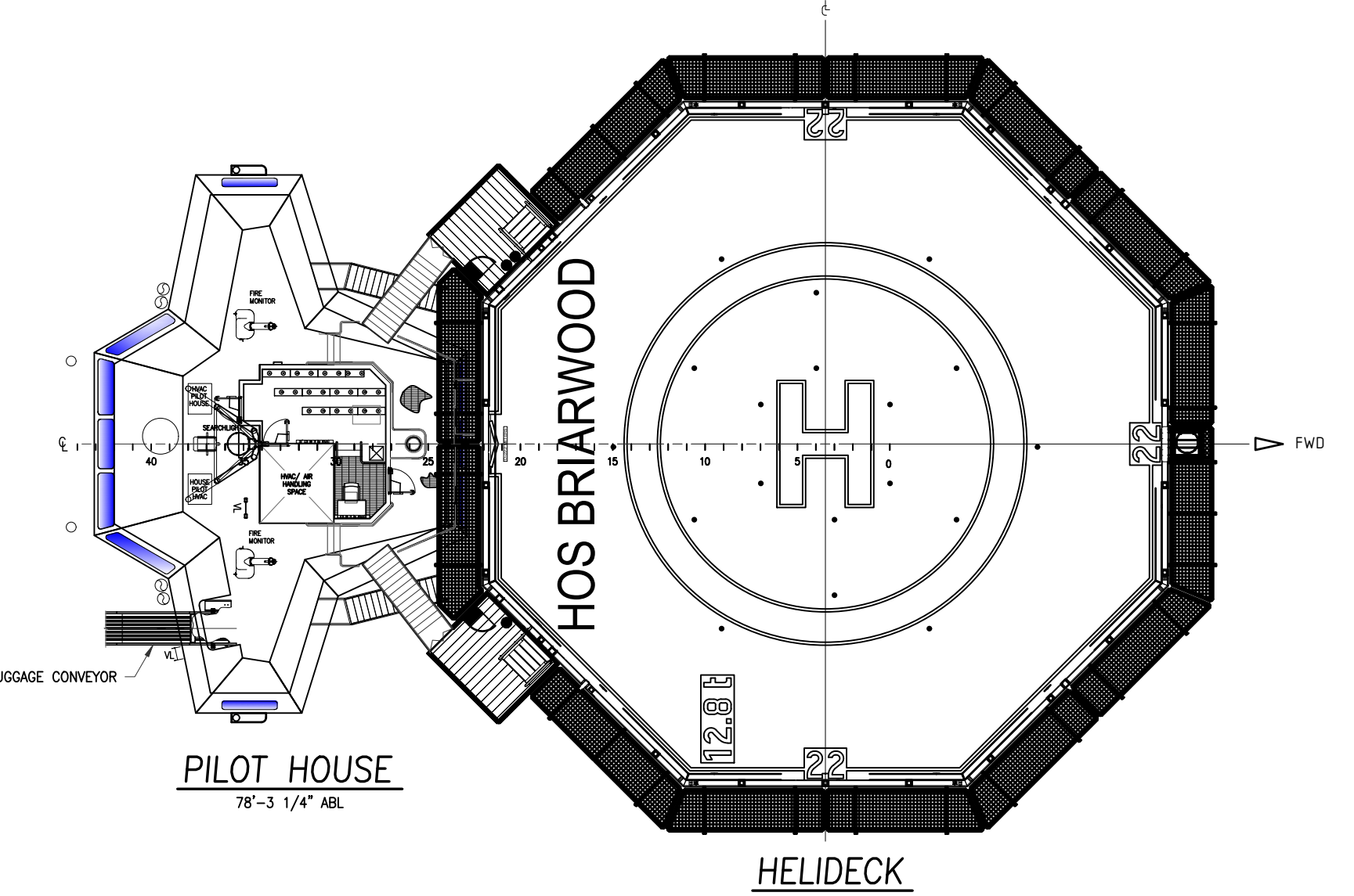
HELIDECK
