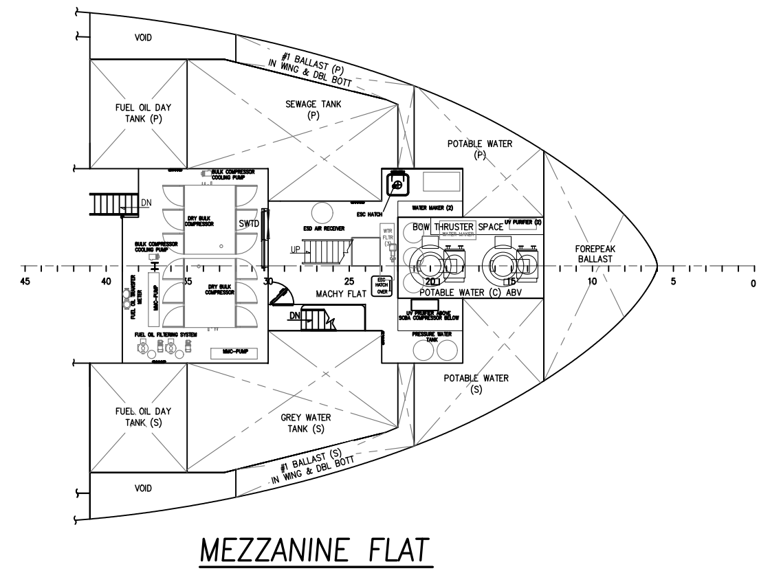
MEZZANINE FLAT
