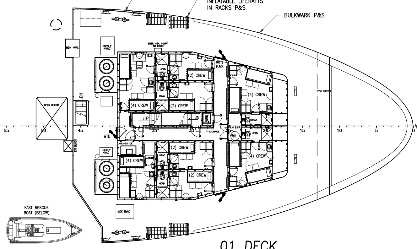
01 DECK
