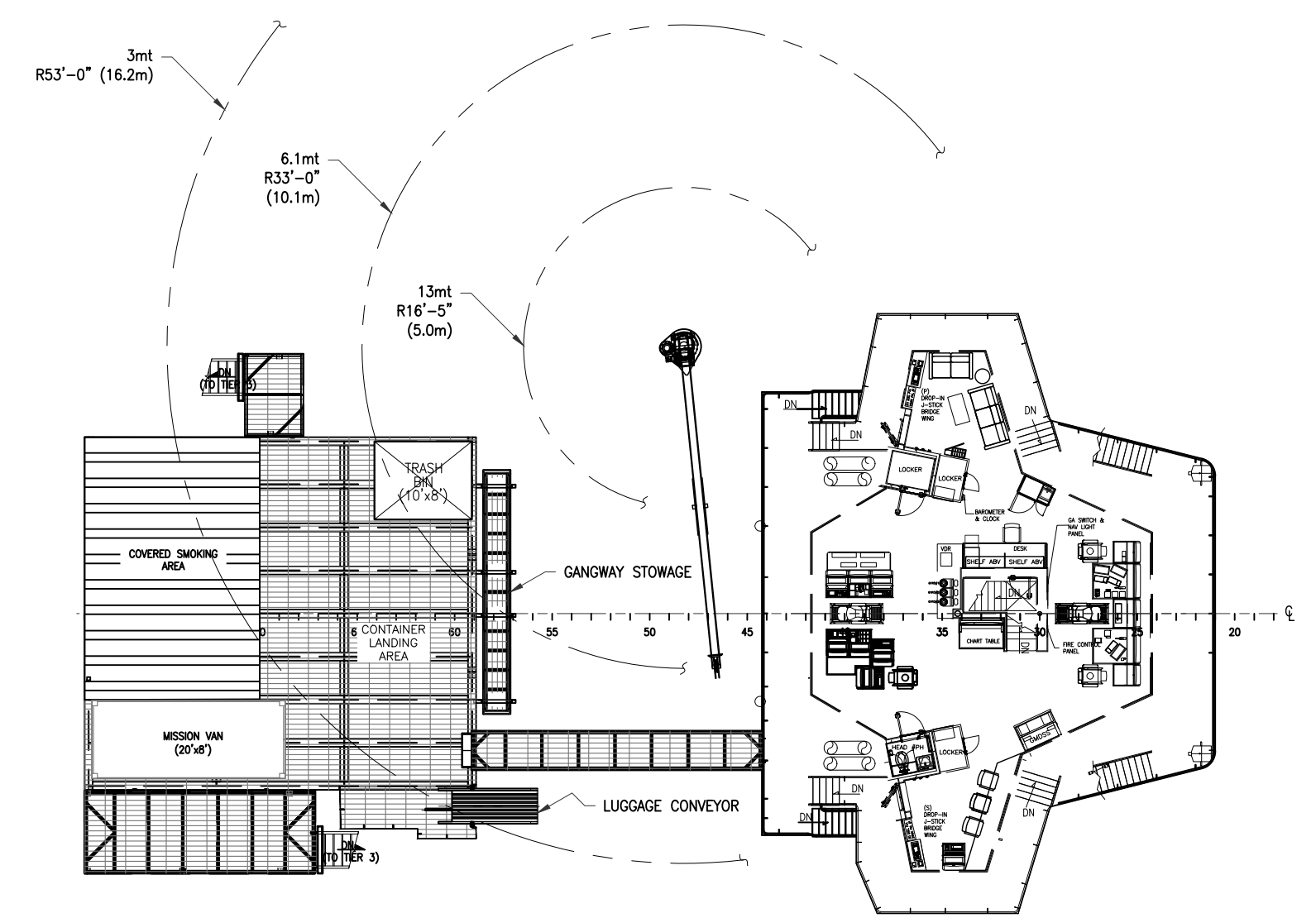
LANDING FLAT
