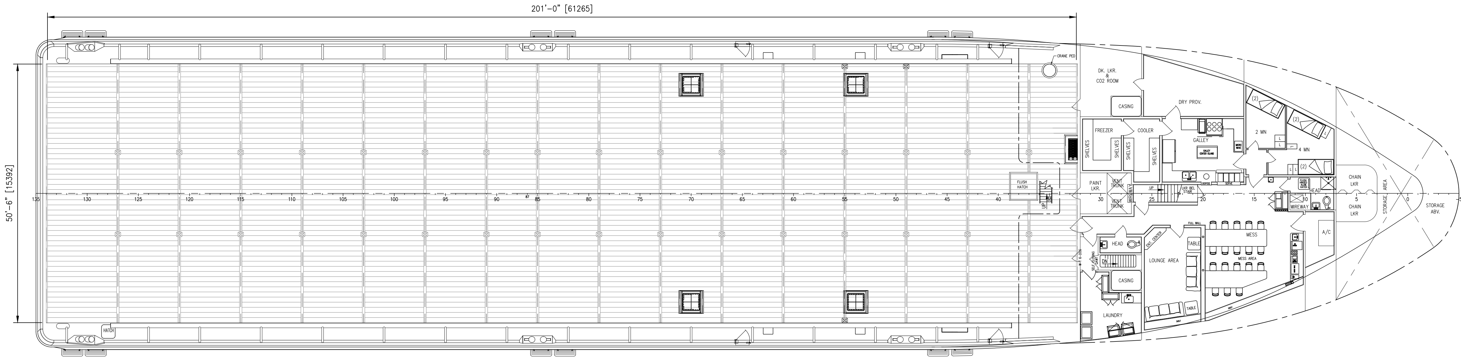
MAIN DECK PLAN
