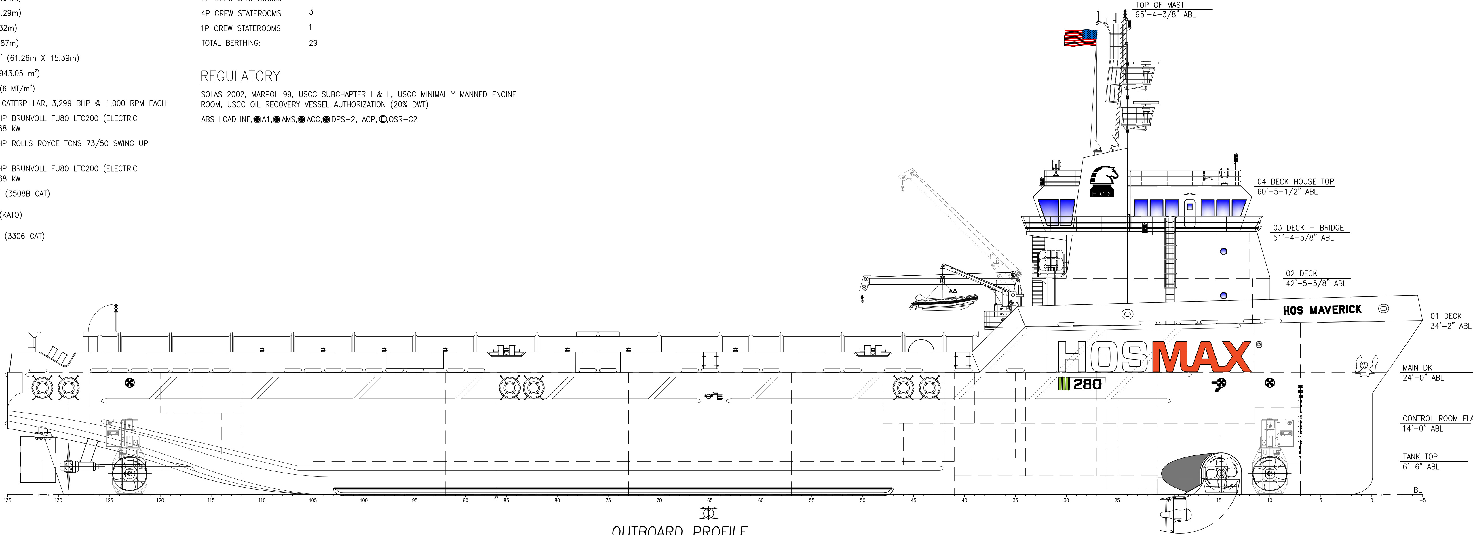
OUTBOARD PROFILE
